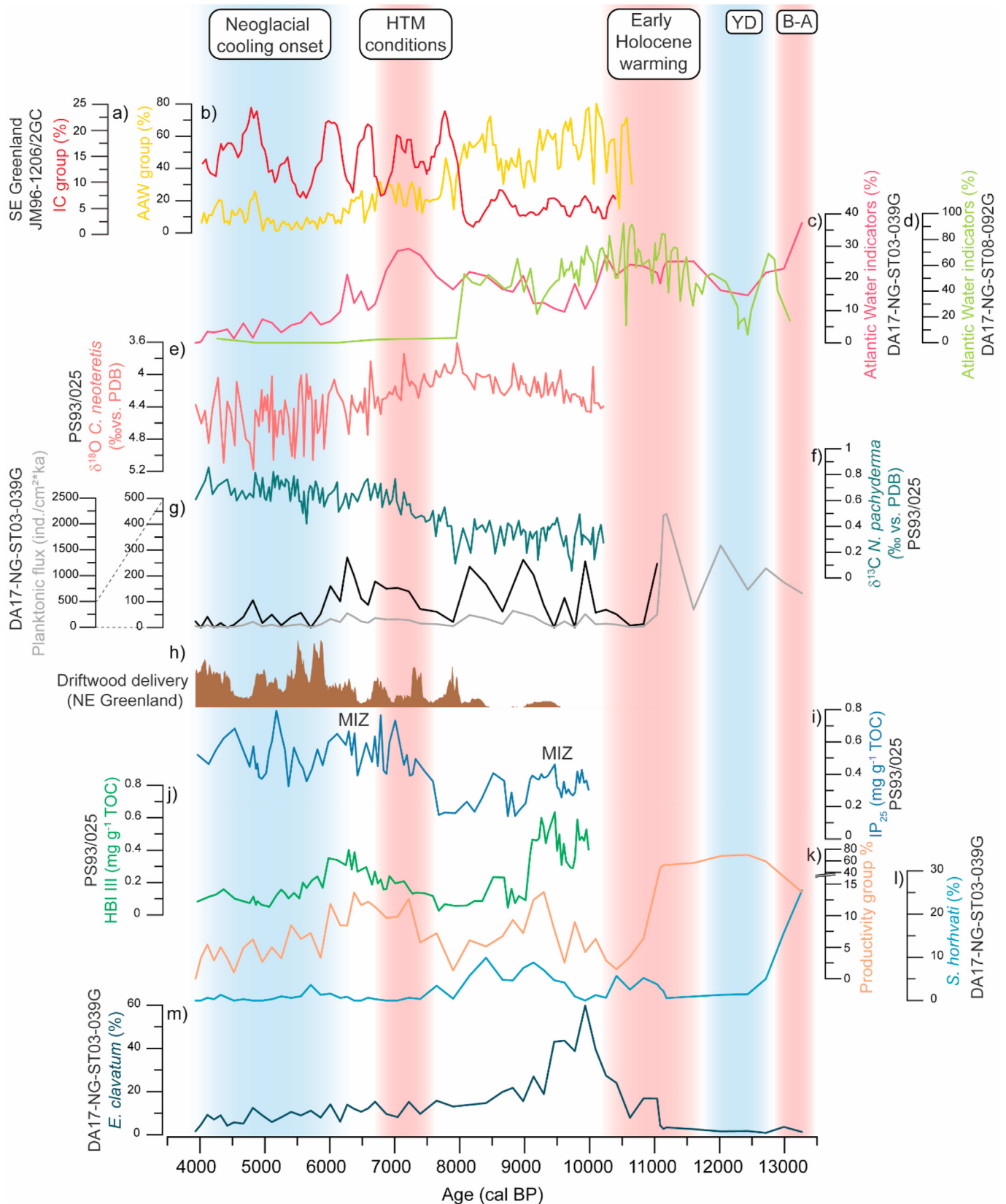
Fig. 8. Comparison between selected foraminiferal data from this study and proxy records from the Fram Strait and Southeast Greenland margin. a) IC group % ( C. neoteretis ) and b) AAW group % ( Melonis barleeanus and I. norcrossi ) from core JM96-1206/2 GC (Perner et al., 2016), c) Atlantic Water group % ( C. neoteretis and I. norcrossi ), d) Atlantic Water indicators % from core DA17-NG-ST08-092G (Davies et al., 2022), e) \delta^{18}\text{O} C. neoteretis and f) \delta^{13}\text{C} N. pachyderma from core PS93/025 (Zehnic et al., 2020), g) the planktonic flux, h) driftwood delivery record from Northeast Greenland (Funder et al., 2011b), i) \text{IP}_{25} and j) HBI III from core PS93/025 (Syring et al., 2020a), k) productivity group % ( S. feylingi , N. labradorica , and E. arctica ), l) S. horvathi %, m) E. clavatum %. MIZ: Marginal ice zone. Chronostratigraphical/climatic intervals are shown at the top (B-A = Bølling-Allerød,
